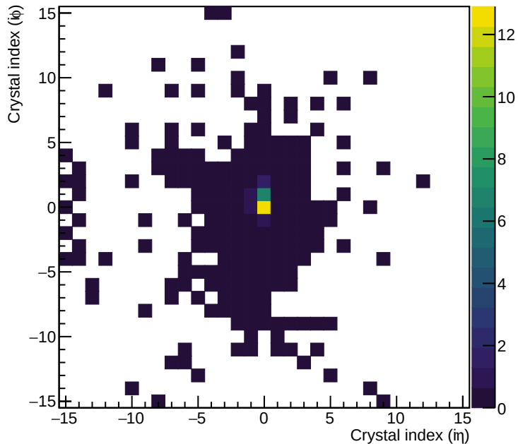
A \rightarrow \gamma\gamma (10 GeV) - Resolved
