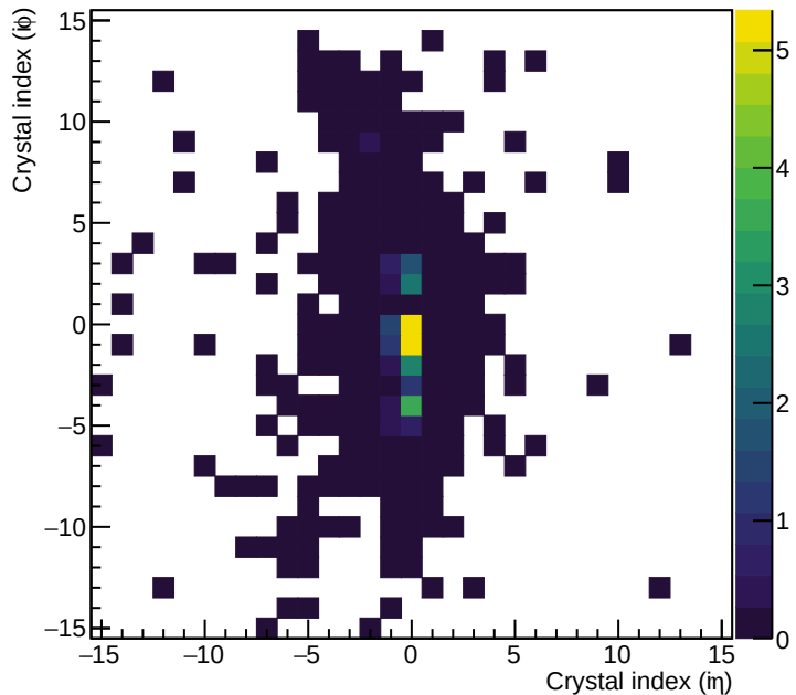
A \rightarrow \gamma\gamma (0.1 GeV) - Merged
